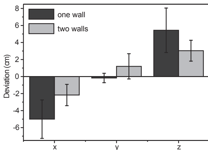
FIG. 7—Deviation for bloodstain selections from one wall (front wall, dark gray) and for bloodstain selections from two walls (light gray). The deviation of the estimated point of origin (PO) from the actual PO is plotted for all three coordinates ( n = 3 ). In the x - and z -direction, selections from two walls distinctly correspond to less deviation. In the y -direction, a slight increase is visible. See text for explanation.
